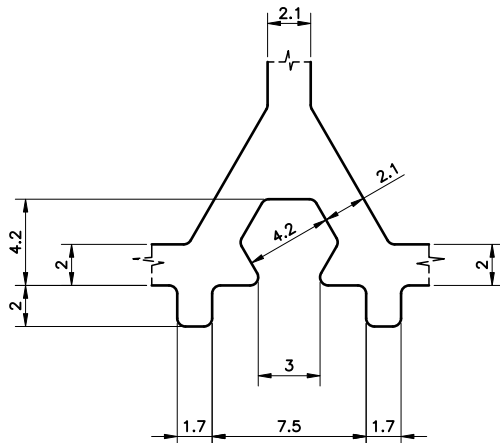
DETAIL C SCALE 4:1
