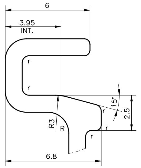
DETAIL A SCALE 6:1
