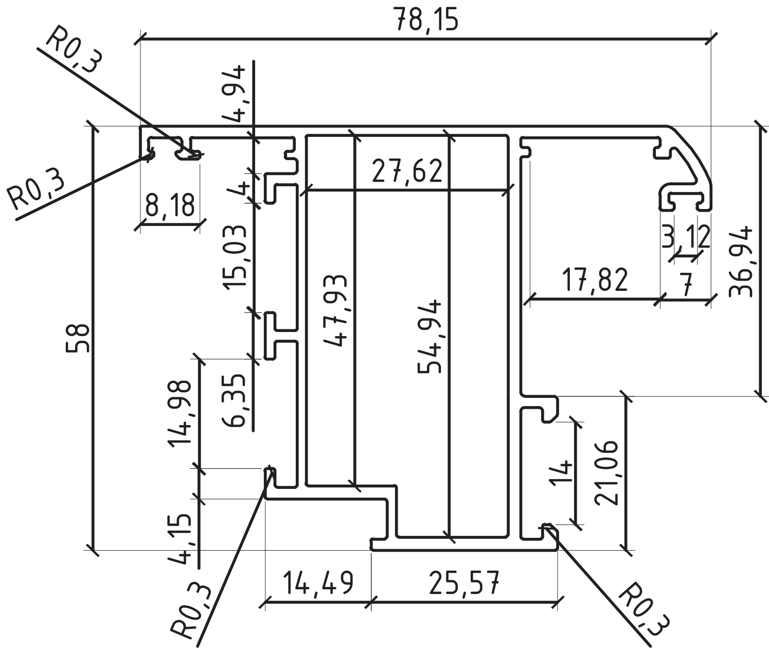
Casement Window Shutter Frame
