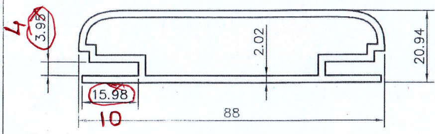
PROPOSAL DRAWING Q02079
