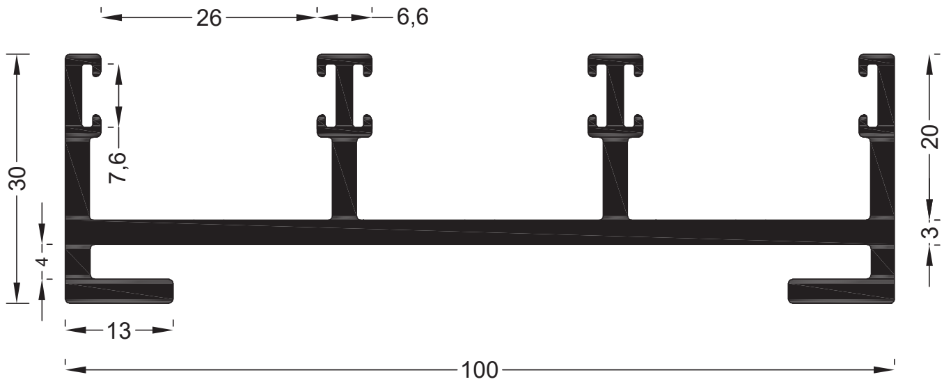
3Track Top/Side 1.7 Kg/M approx
