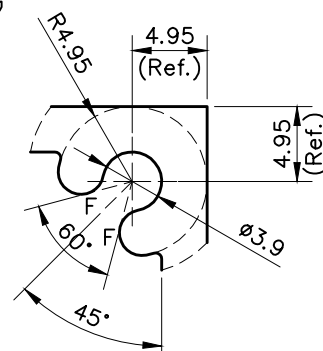
DETAIL B SCALE 2:1
