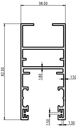
Single Glass Sliding Sash
