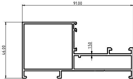
2 Track Fix Profile
