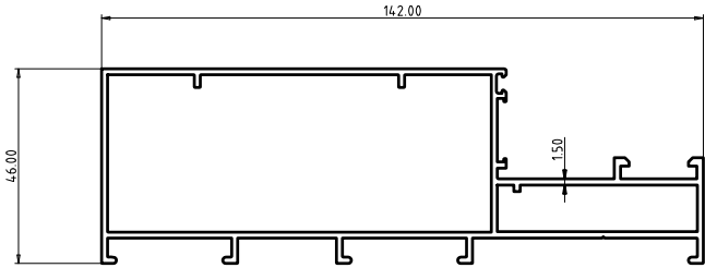
2 Track Fix Profile
