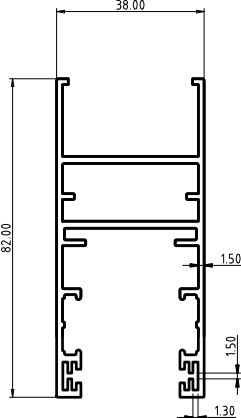
DGU Glass Sliding Sash
