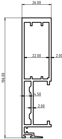
Hurricane Slim Interlock
