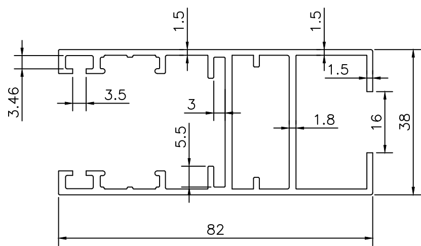
Single Glass Sliding Sash
