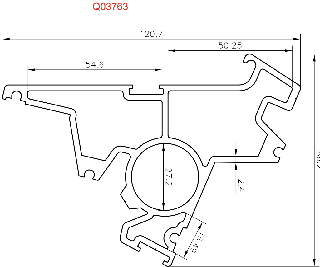
ALP4-RTRUSS
