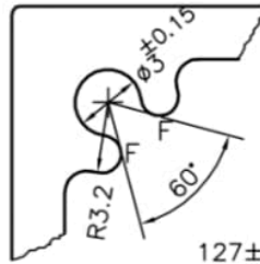
DETAIL OF "A" SCALE 3:1
