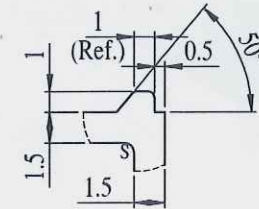
DETAIL A SCALE 4 : 1
