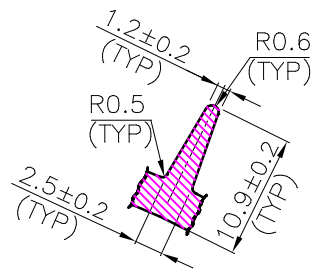
DETAIL-B SCALE 1.5:1
