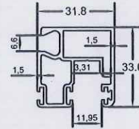
84218 MESH SASH PROFILE
