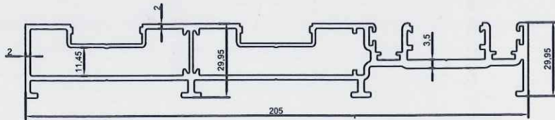
84116 3 Track Vertical Frame Profile
