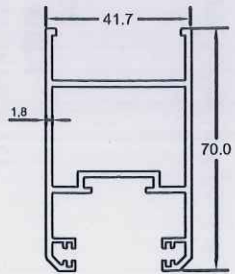
84216 HANDLE SECTION SASH
