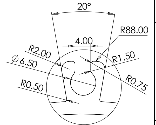
DETAIL F SCALE 2 : 1
