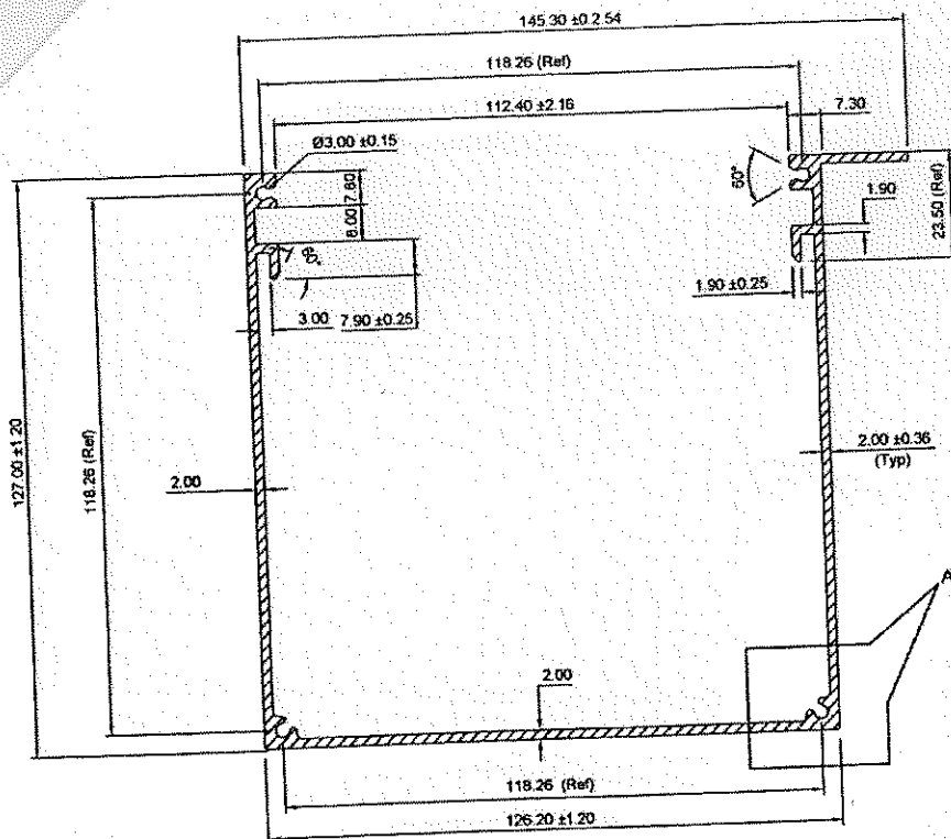
DETAILED SECTION DRAWING (SCALE - 1 : 1)
