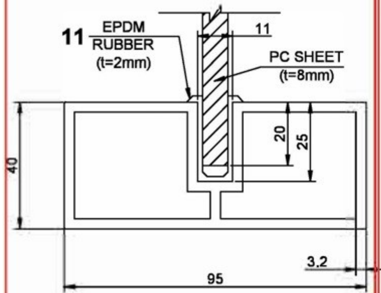
DETAIL - D (SCALE N.T.S.) ALUMINIUM SECTION (SINGLE EXTRUDE)
