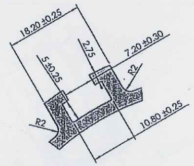
DETAIL A SCALE 2 : 1.5
