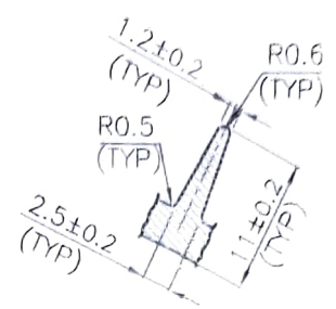
DETAIL-'B' SCALE 1.5:1
