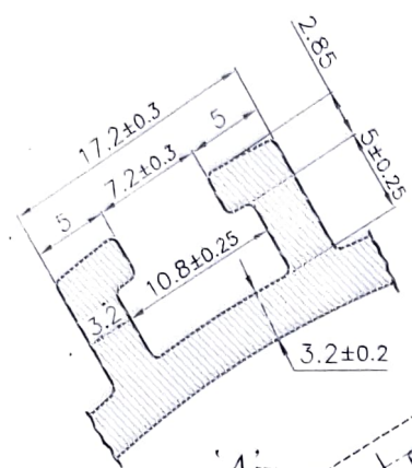
DETAIL-'A' SCALE 2:1
