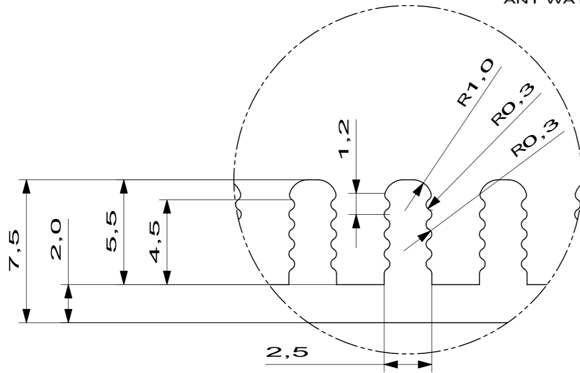
DETAIL A SCALE 5:1
