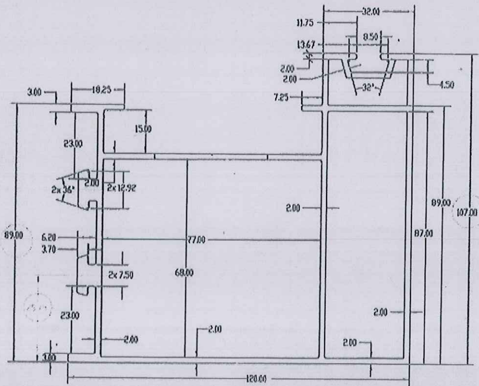
Front View Scale 1:50
