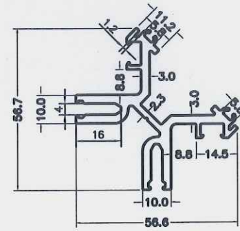
Corner Section
