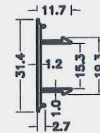
Cover Cap
