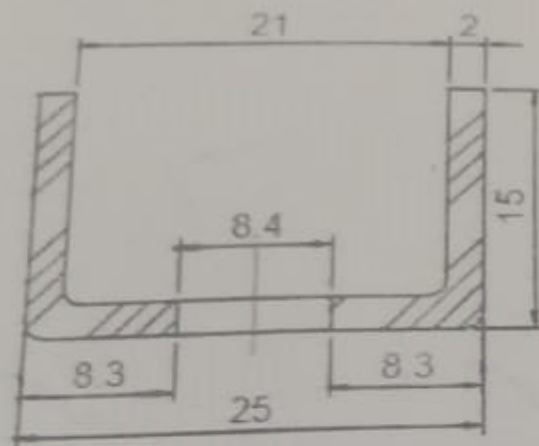
ALUMINUM WASHER DETAIL
