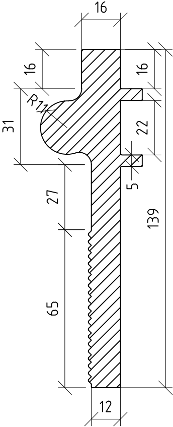
HOOK BRACKET
