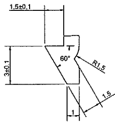
DETAIL B SCALE 5.000
