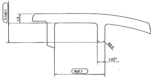
DETAIL C SCALE 5.000
