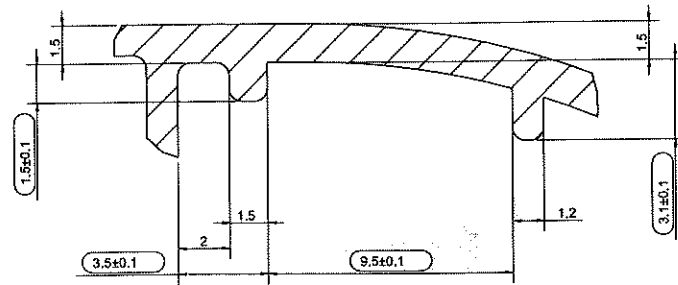
DETAIL C SCALE 5.000
