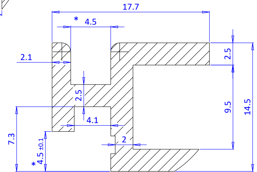
DETAIL F SCALE 4 : 1
