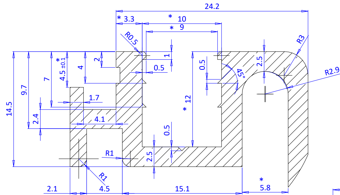
DETAIL E SCALE 4 : 1
