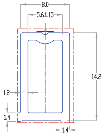
DETAIL-A SCALE 4 : 1
