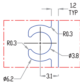
DETAIL-A SCALE 4 : 1
