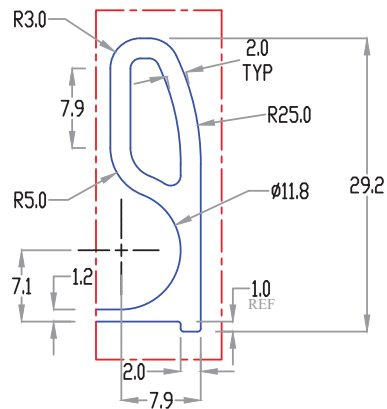
DETAIL-A SCALE 2 : 1
