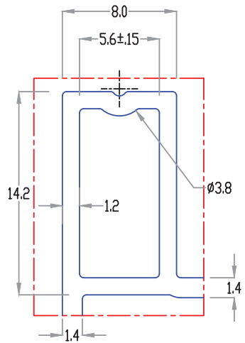
DETAIL-A SCALE 4 : 1
