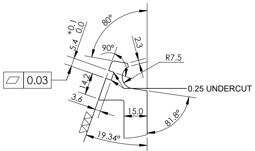
DETAIL A SCALE 2 : 3
