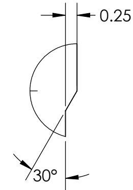
DETAIL B SCALE 12 : 1
