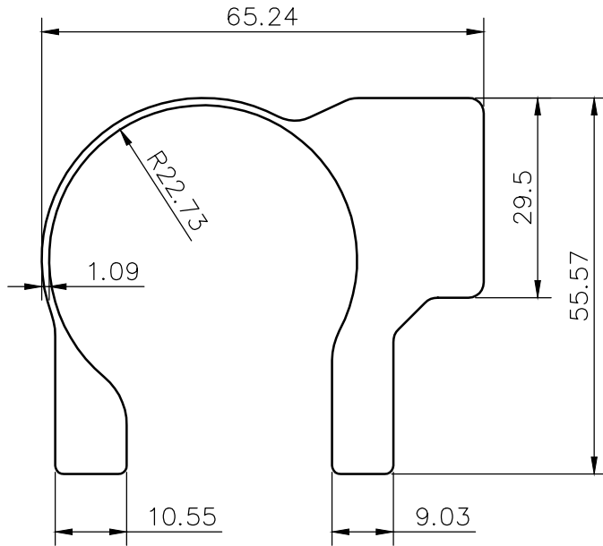
CUSTOMER DRAWING
