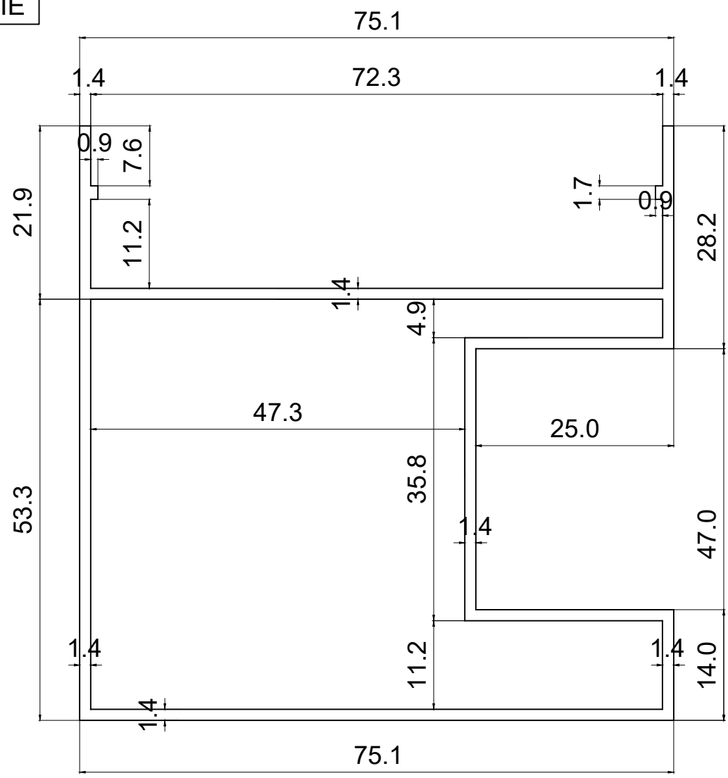
NEW DIE FOR COUNTER DRAWING ( K S V COVER PLATE SIDE-02 )
