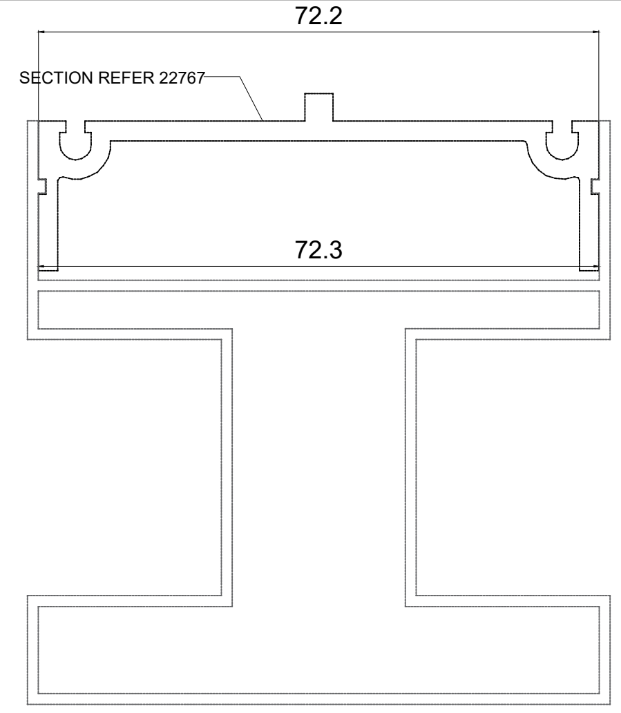
FIXING DETAIL FOR 22767
