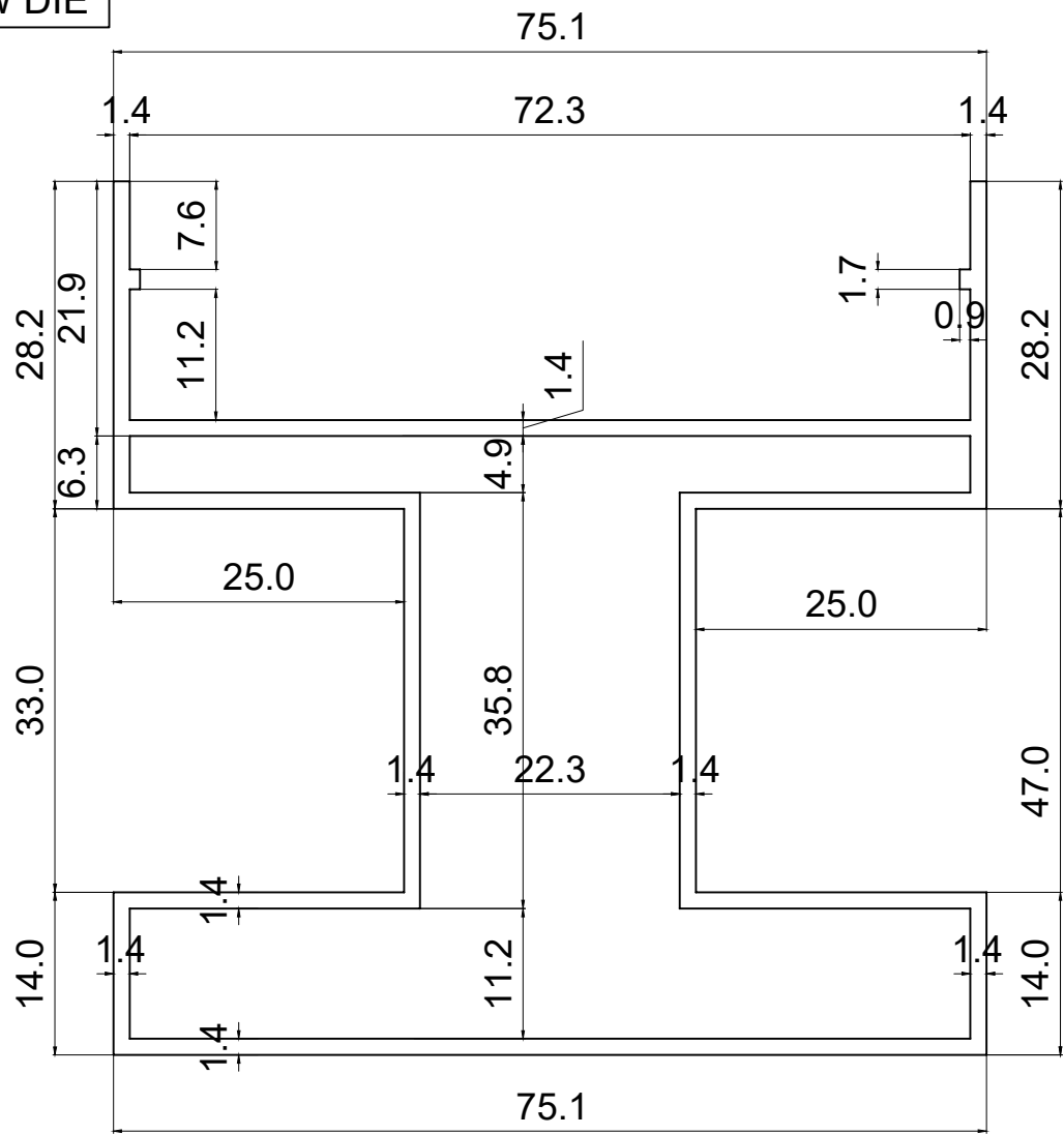
NEW DIE FOR COUNTER DRAWING ( K S V COVER PLATE MID-01 )
