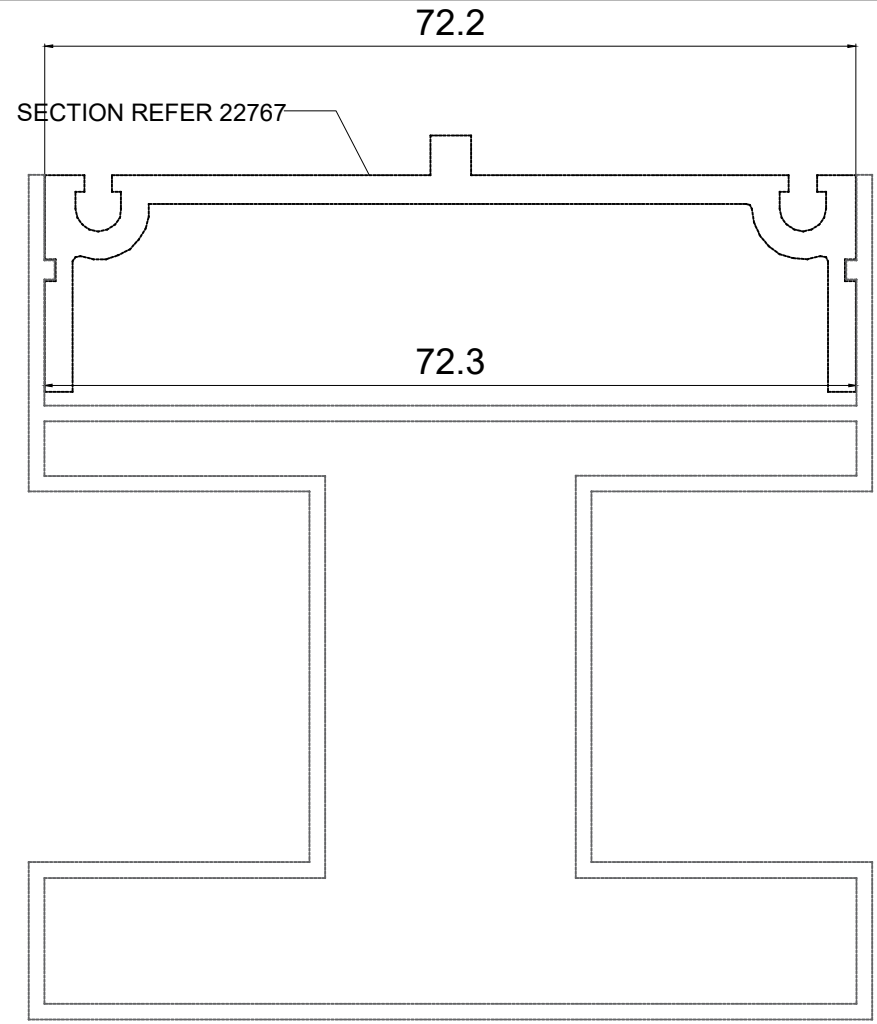
FIXING DETAIL FOR 22767
