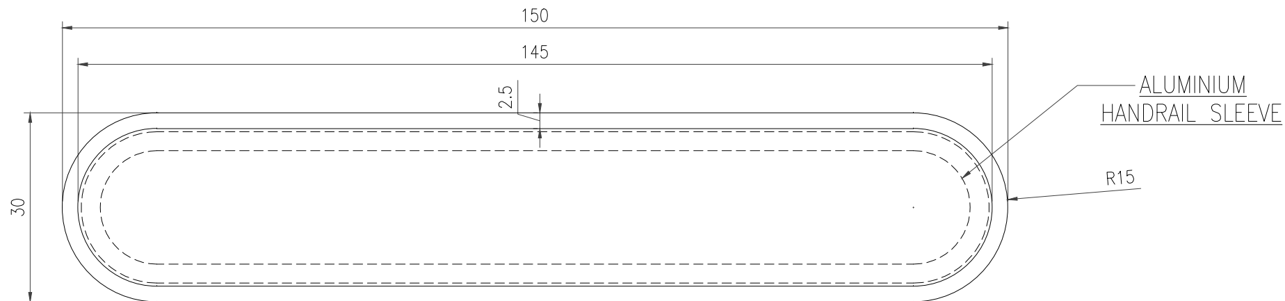
ALUMINIUM HANDRAIL ALLOY-6063-T6 WEIGHT-2.211 Kg/Mtr.
