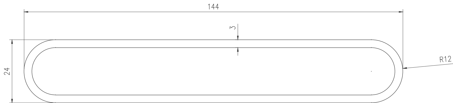
ALUMINIUM HANDRAIL SLEEVE ALLOY-6063-T6 WEIGHT-2.487 Kg/Mtr.
