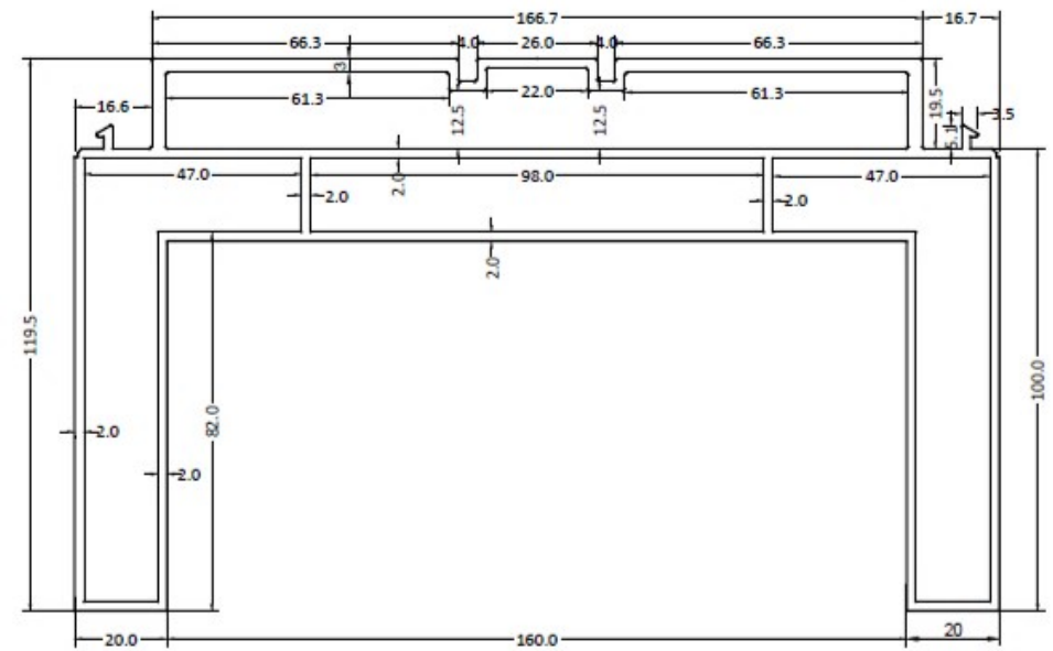
Cover Profile (AXS-C200)
