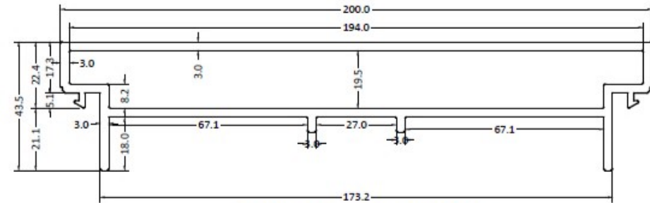
Outer Pressure Profile AXS-P200)
