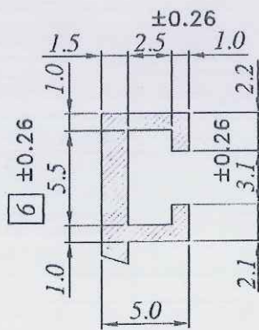
DETAILS AT-A
