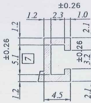
DETAILS AT-B
