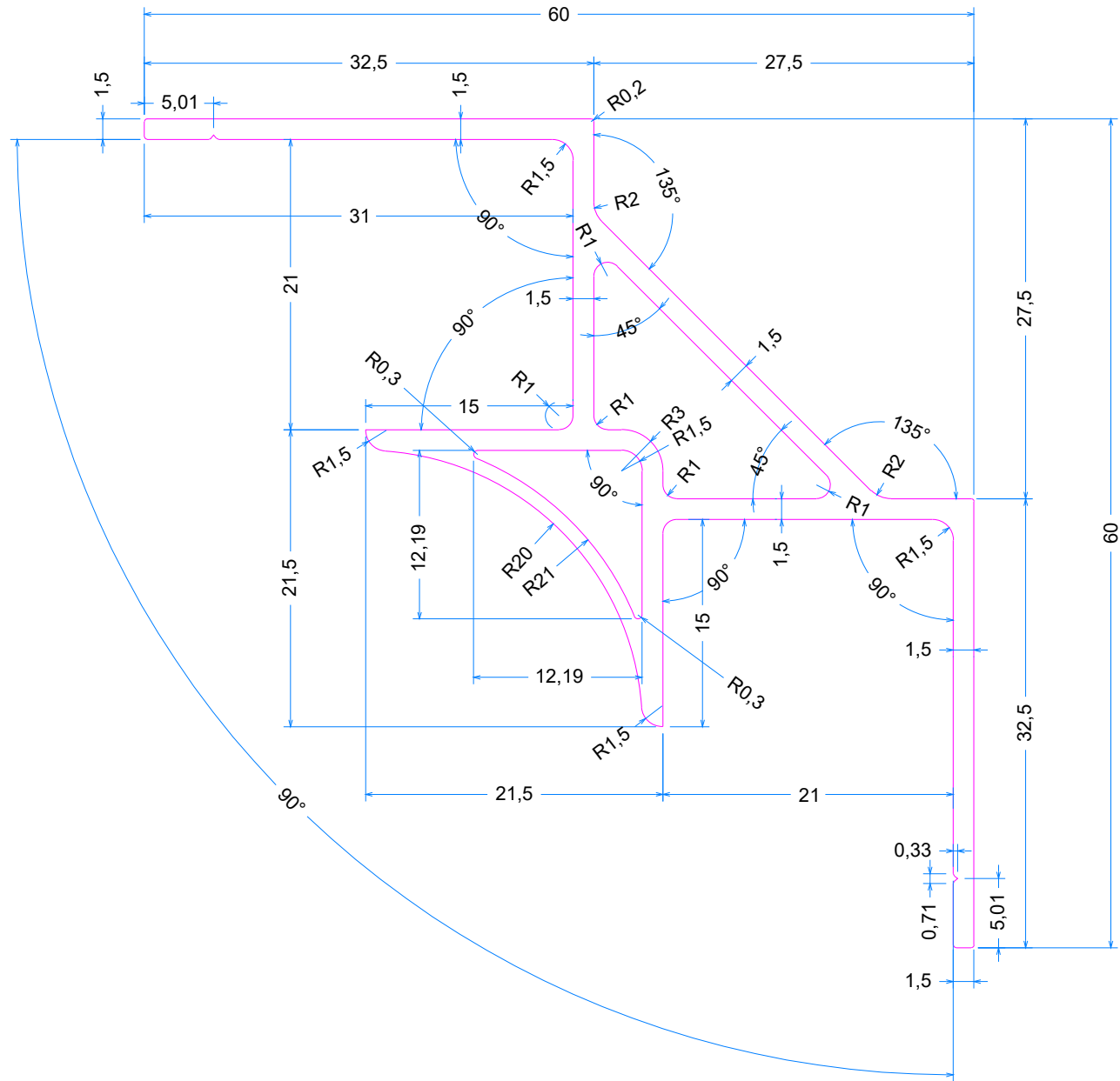
NAME - 90 DEGREE EXTRUSION PROFILE MATERIAL - ALUMINUM
