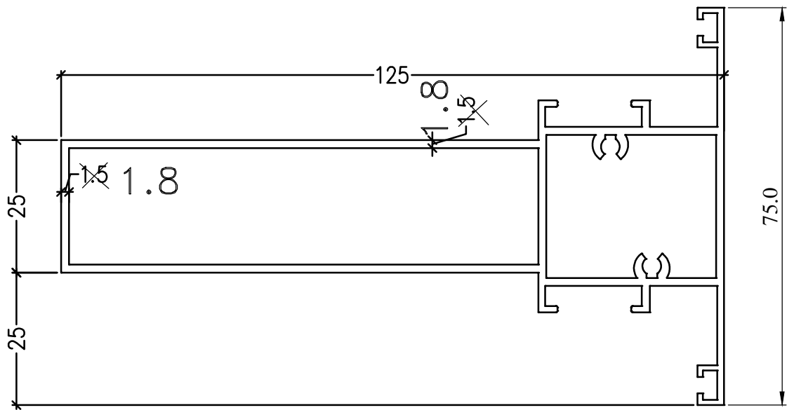
CD2 Mullion
