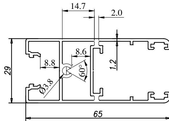
SH SLIDING HANDRAIL SHUTTER
