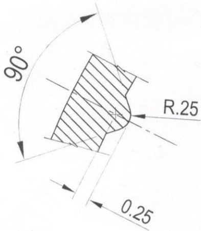
DETAIL "A" (TYP. 2)
