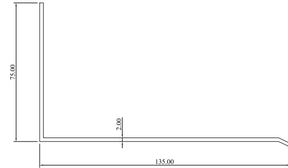
SNPK-400 CORNER PLATE
