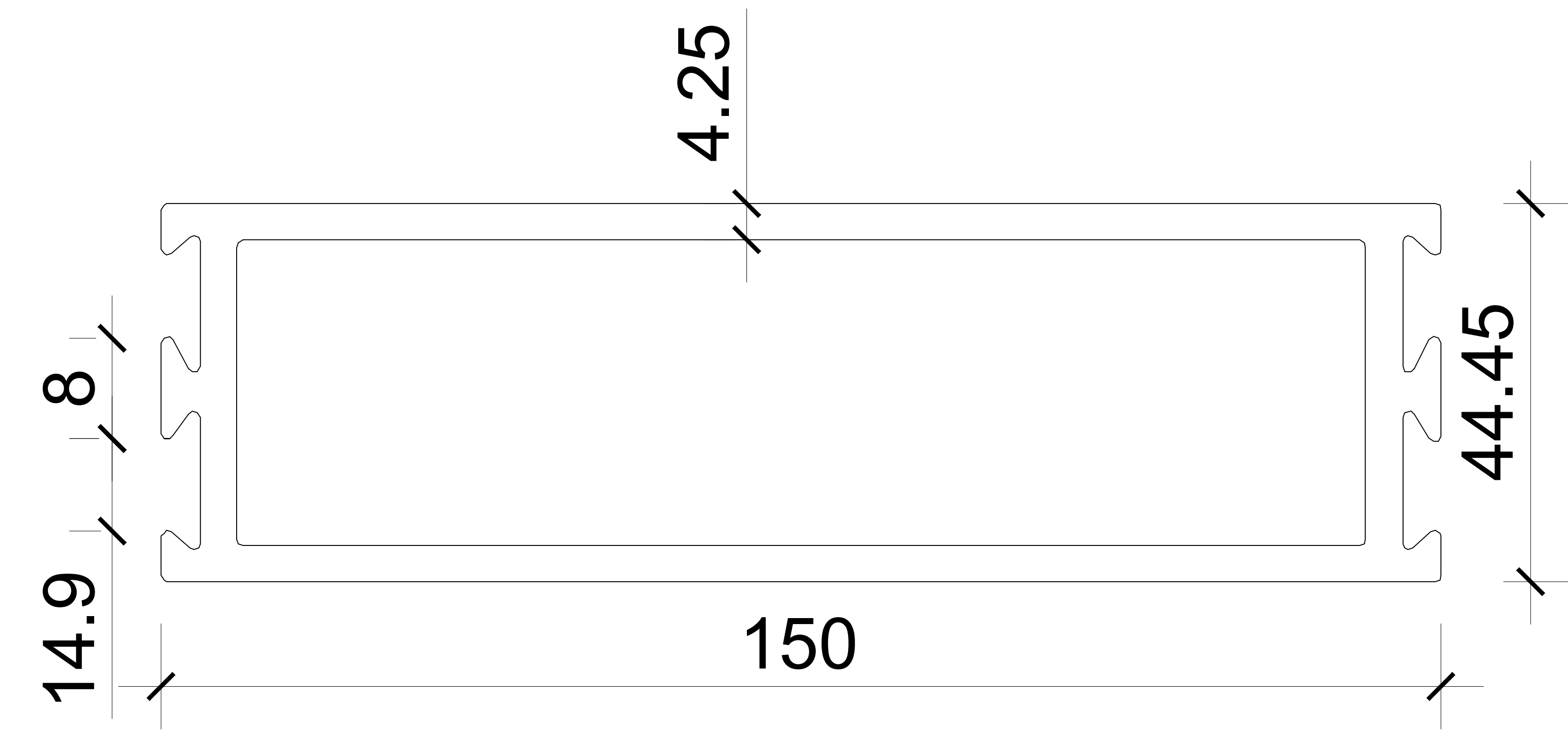
LOCK RAIL SECTION – 19596 (150X44.45X4.25MM)
