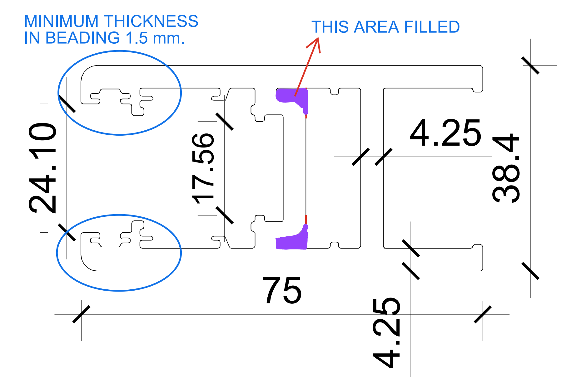
SHUTTER SECTION – P-20060 (75X38.4X4.25MM)
