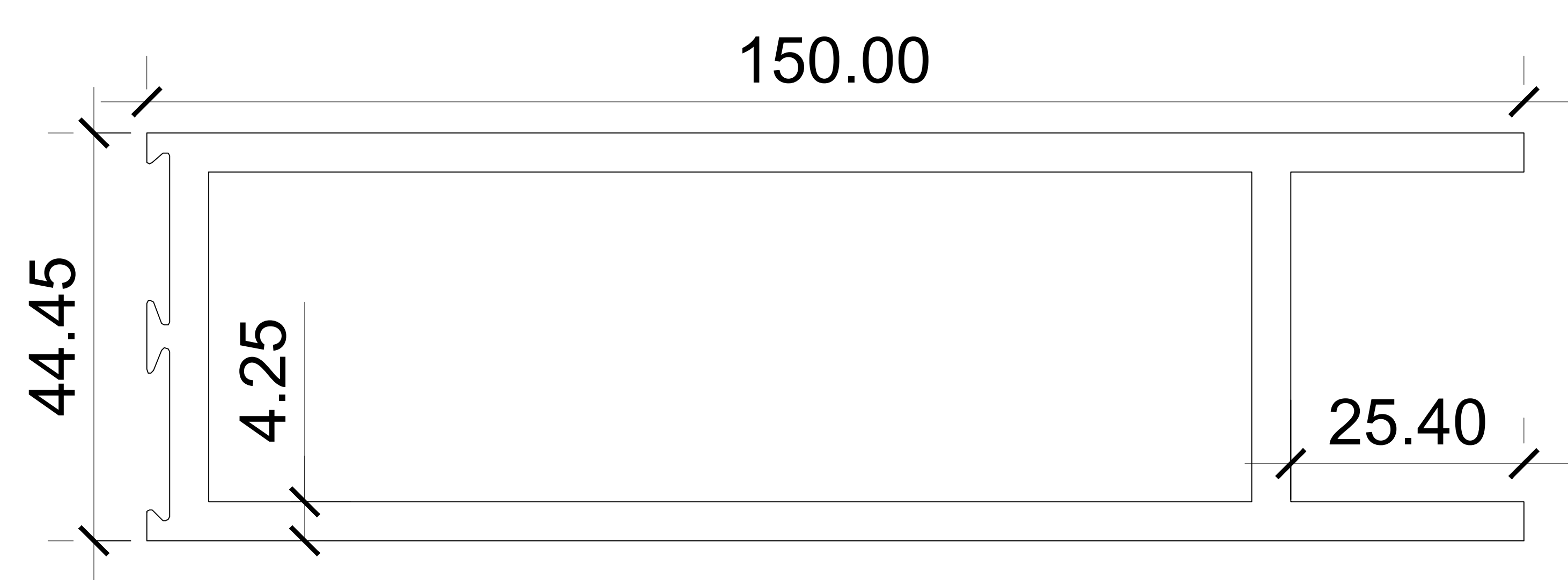
BOTTOM SHUTTER SECTION – 19584 (150X44.45X4.25MM)
