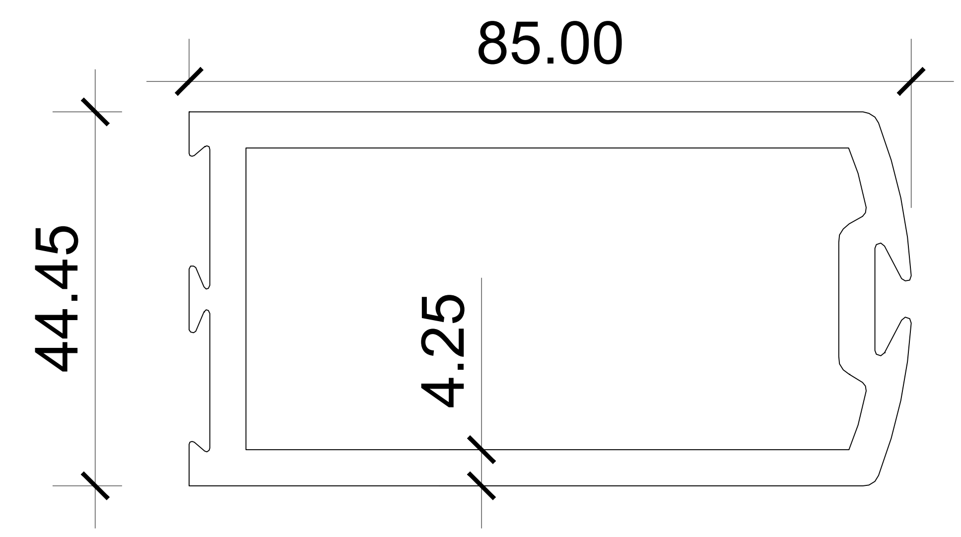
MIDDLE SHUTTER SECTION – 19592 (85X44.45X4.25MM)
