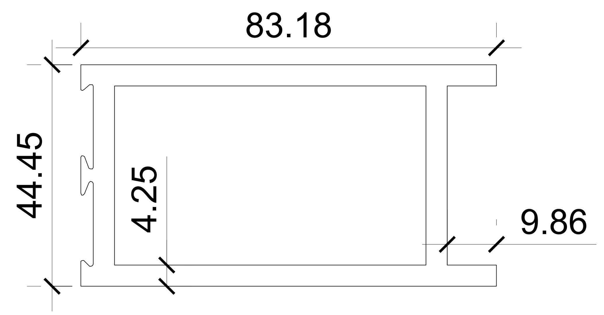
SIDE JINDAL SECTION – 19593 (83.5X44.45X4.25MM)
