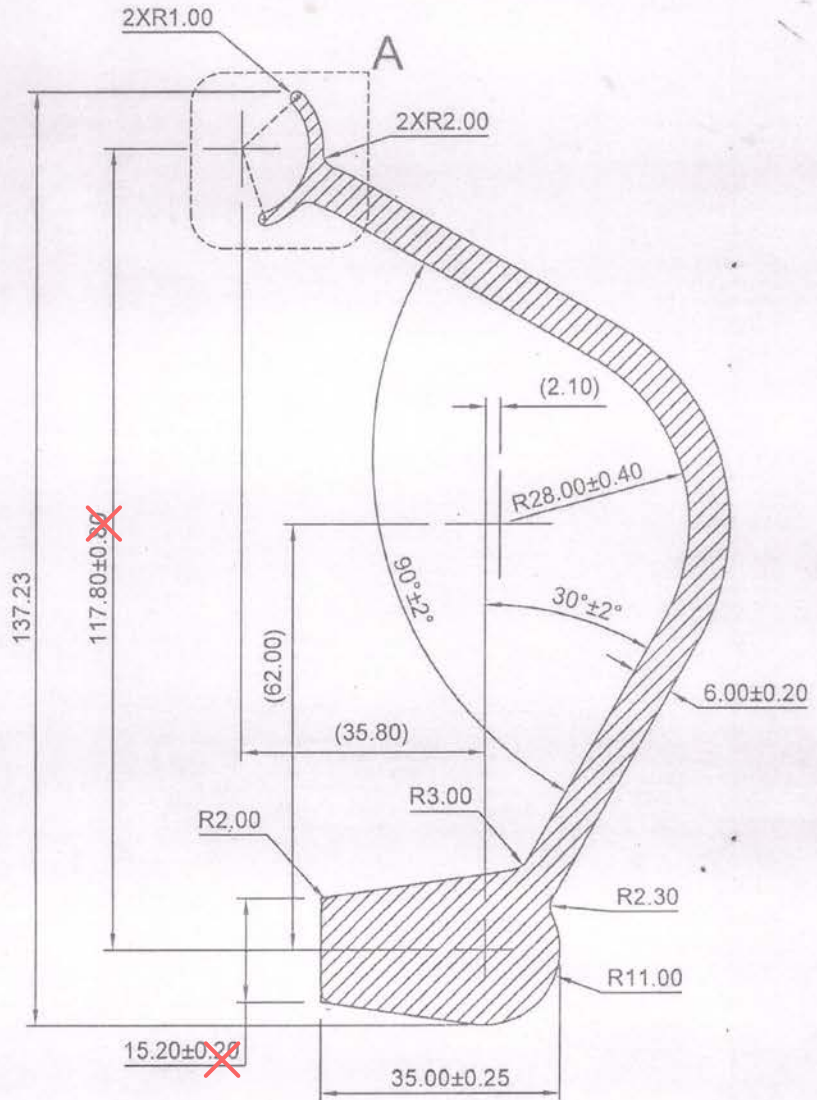
DETAILED SECTION DRAWING (SCALE - 1 : 1)
