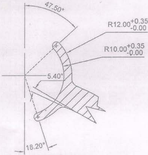
DETAILED SECTION DRAWING OF " A " (SCALE - 2 : 1)
