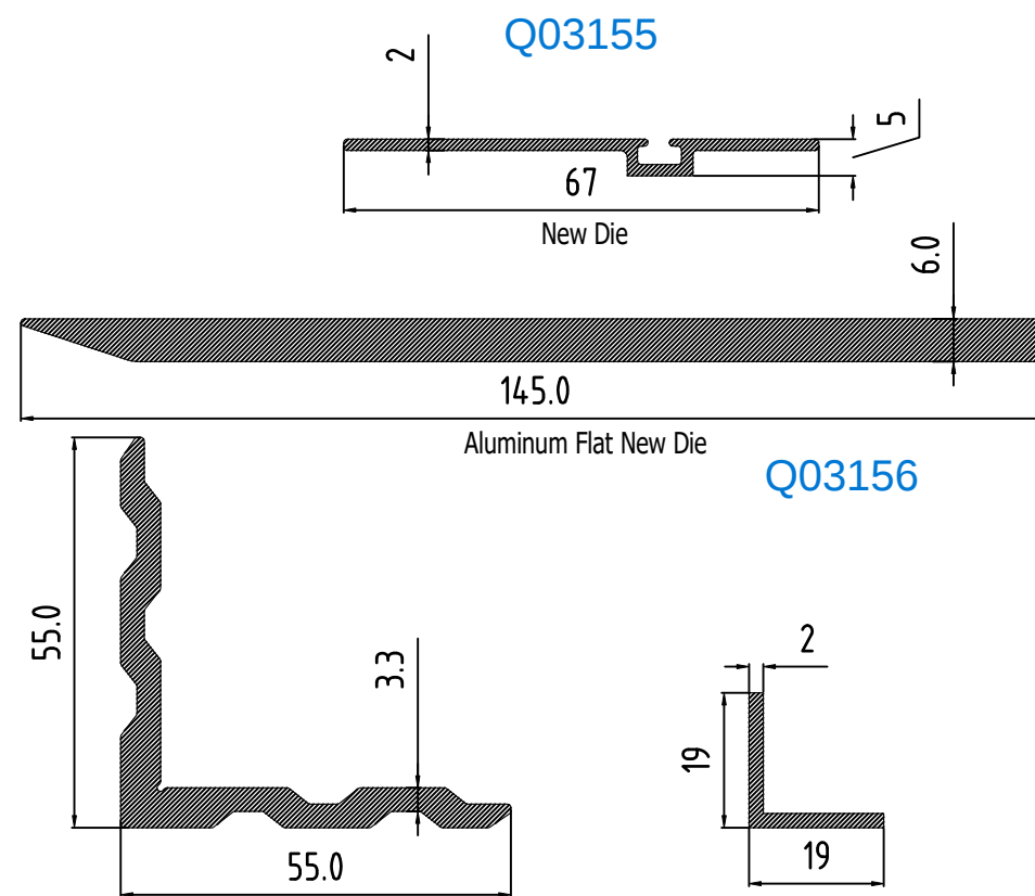
Crimping Cleat Sec no - 35821
