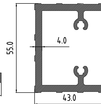
Transom Connector Sec no - 36422
