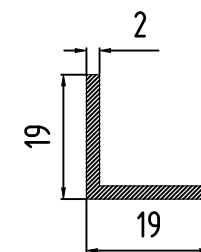
Aluminum Angle Sec no - 16478
