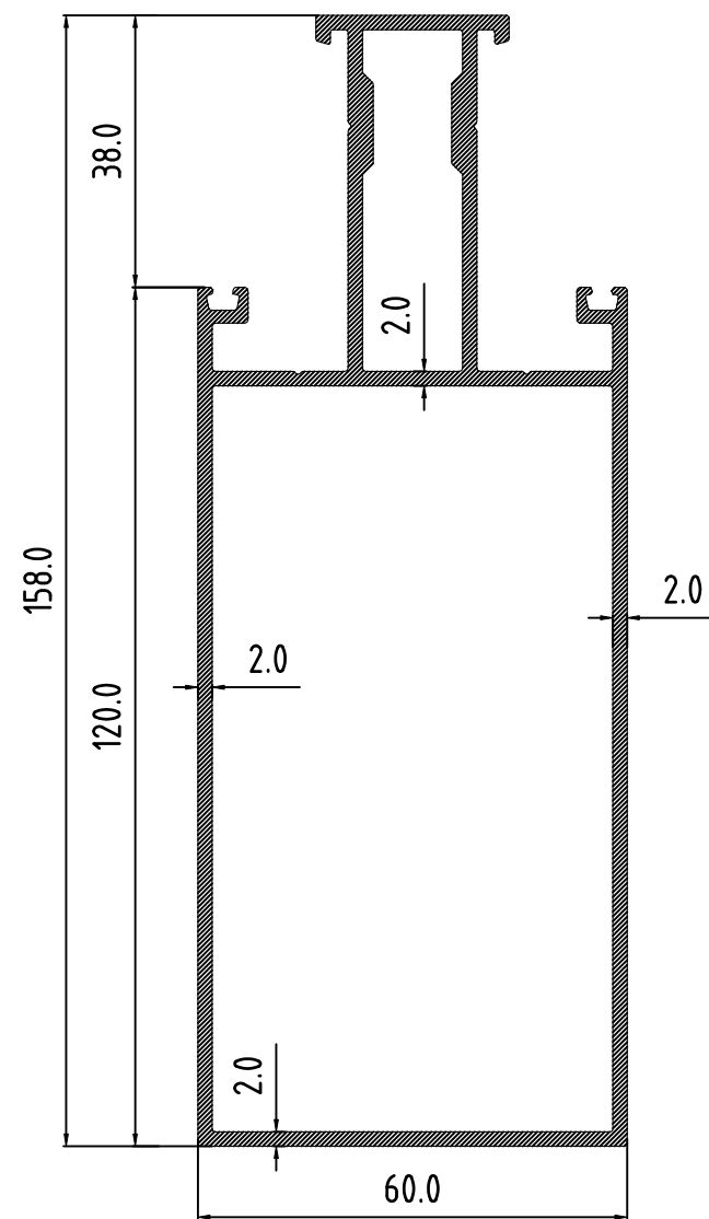
Mullion / Transom Sec no - 29161
