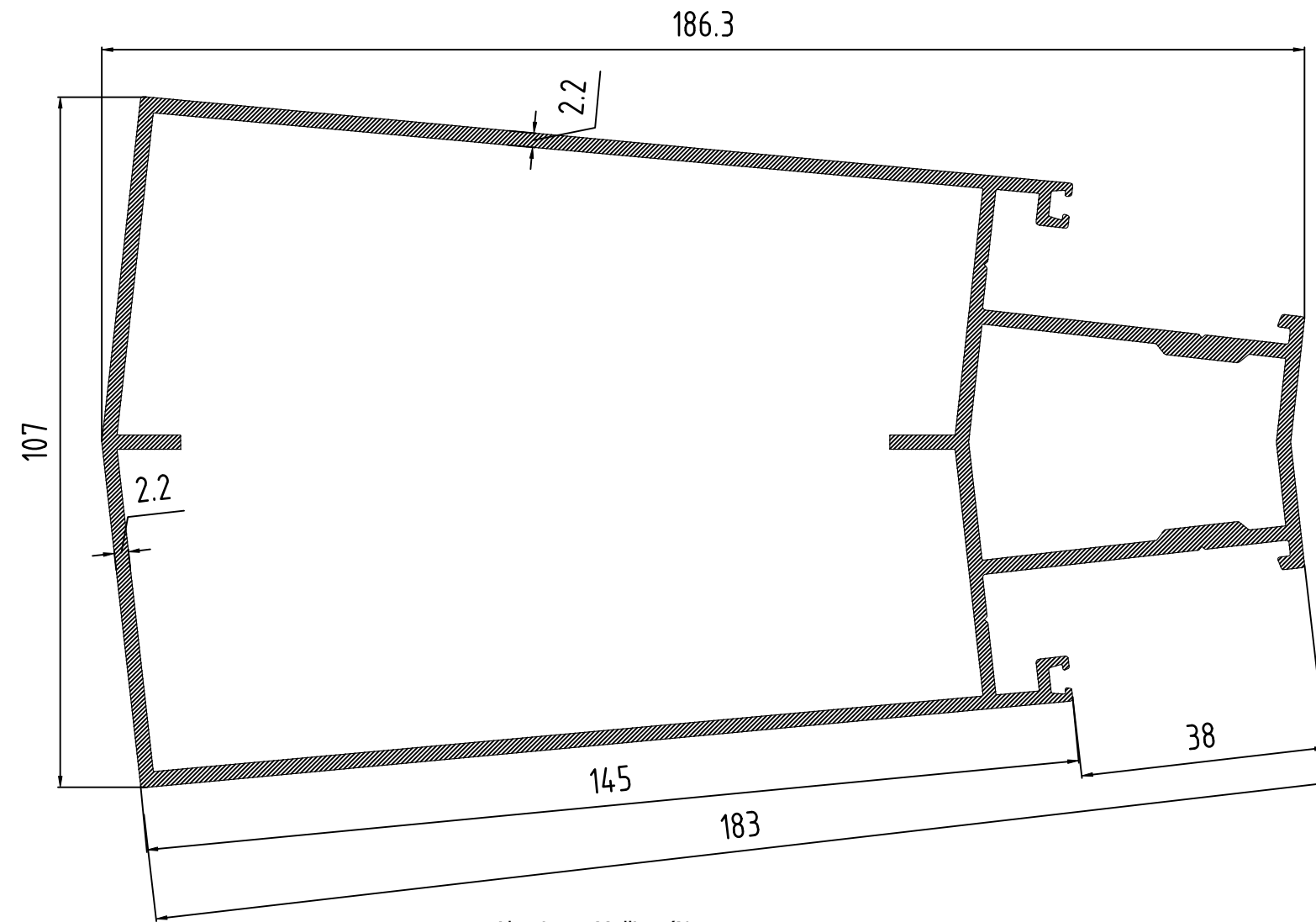
Aluminum Mullion (New Die No - Q03157)
