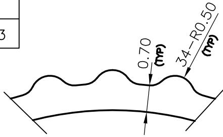
DETAILS "A" SCALE 10:1
