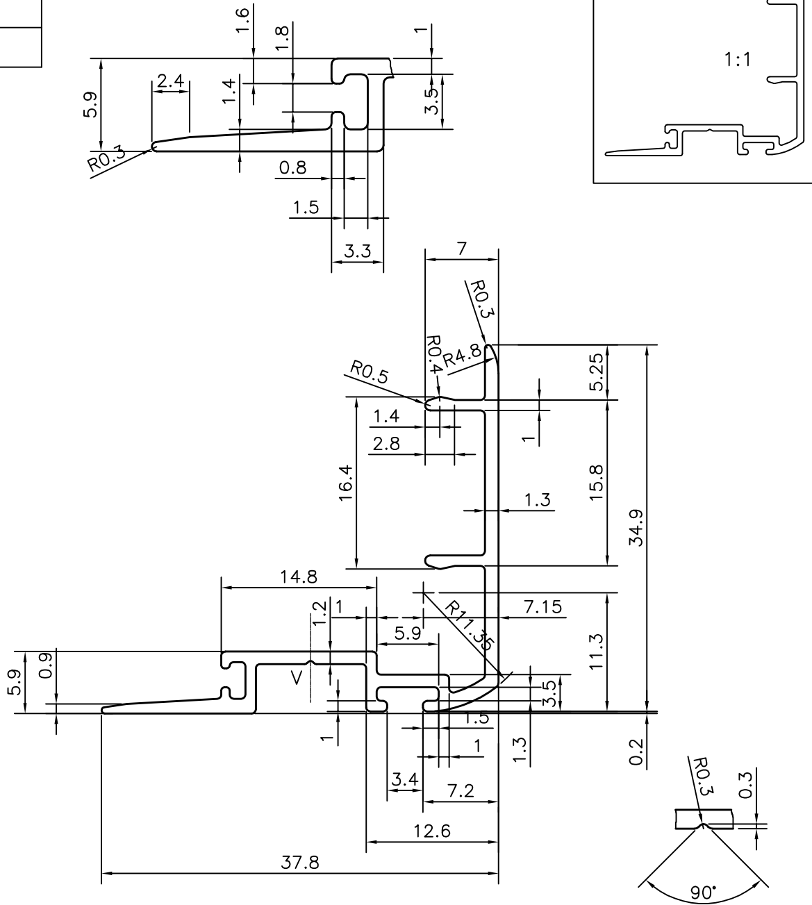
V GROOVE DETAIL
