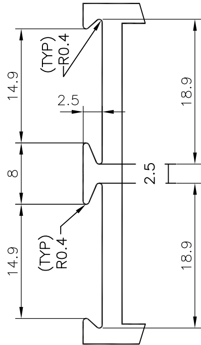
DETAILS - A (2:1)
